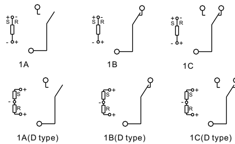
S:Set R:Reset Wiring diagram(Bottom view)
