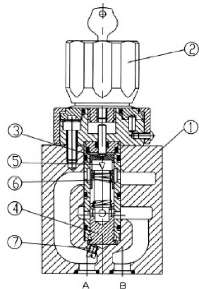
Type 2FRM6B36-20B/...M...
