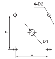
LW26-160 Installation
