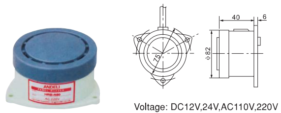
Voltage: DC12V,24V,AC110V,220V
