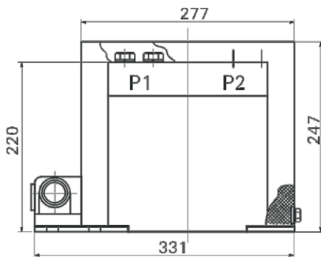
LZZBJ9-12(AS12/175b/2S)
