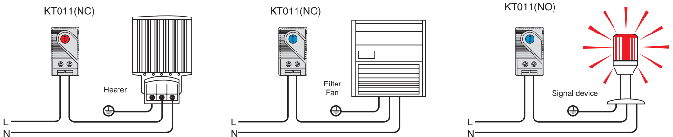
Wiring examples
