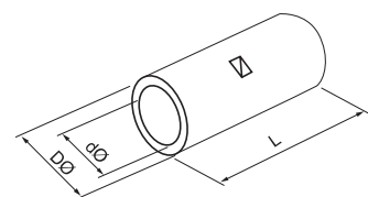
Butt Terminal
