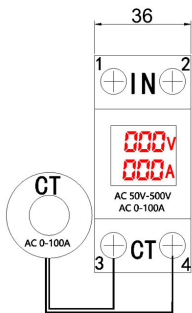
100A CT External
