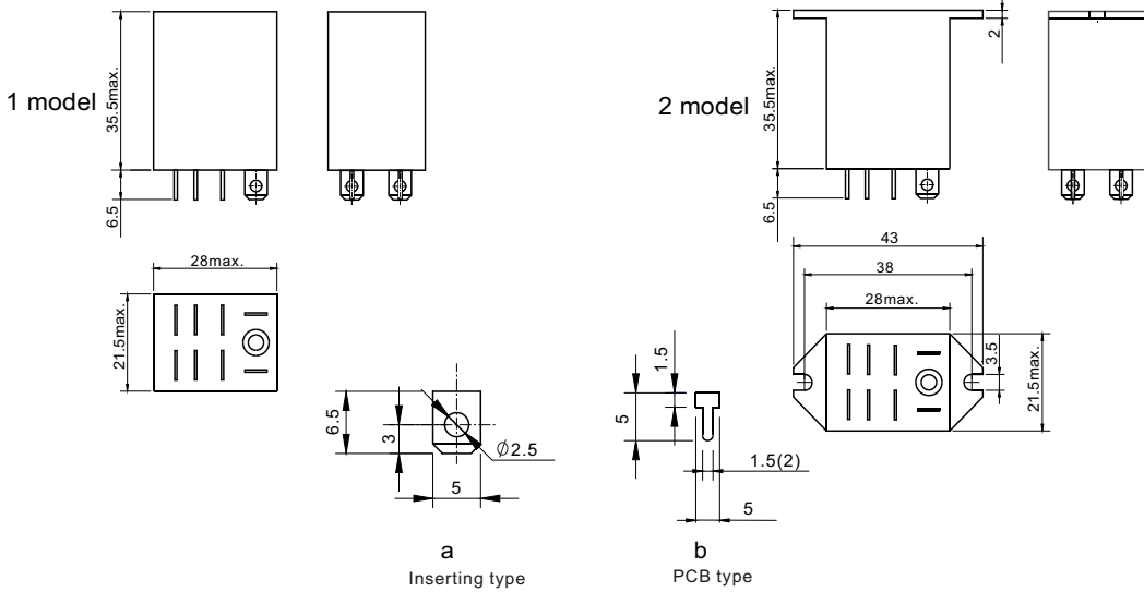
a Inserting type b PCB type Leading end shape diagram Dimensions
