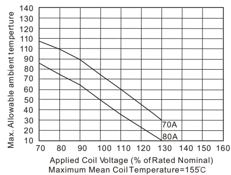
Ambient Temperature vs Coil Voltage for Continuous Contact Load
