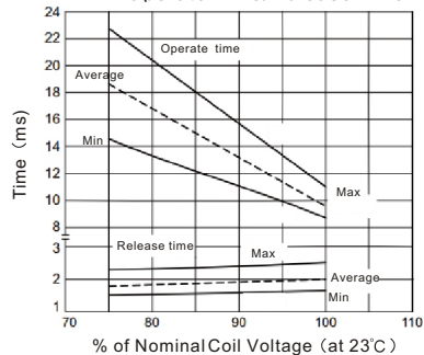
Operate Time/Release Time
