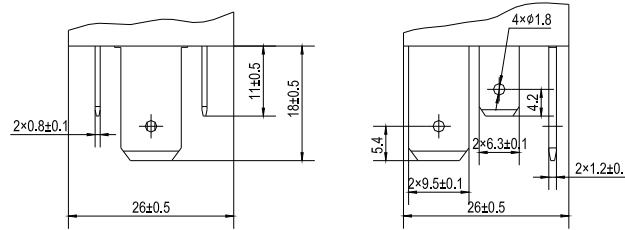
Plug in type Mounting (Bottom view)
