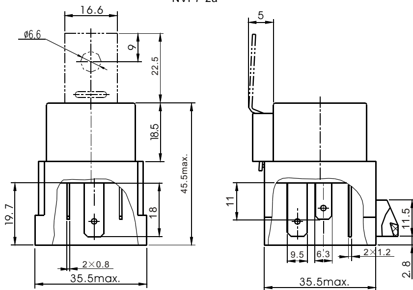
NVF7-2b Dimensions
