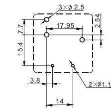
Wiring diagram(Top view)
