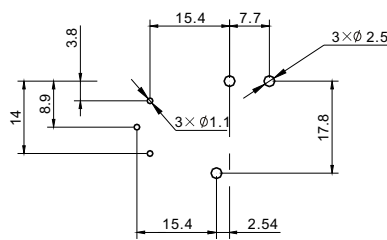
Double coils
