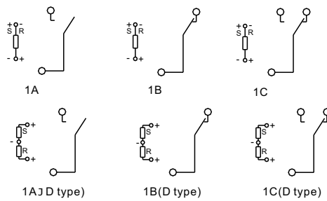
Mounting (Bottom view)
