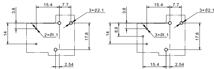
Single coil
