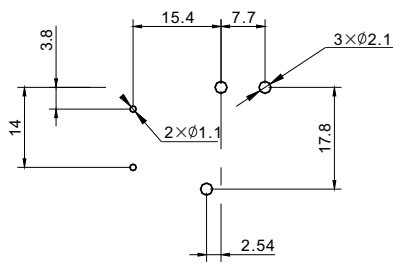
Single coil
