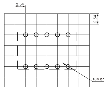
Tolerance: \pm 0.1 Mounting (Bottom view)
