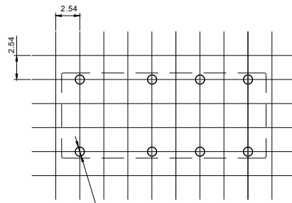
Mounting (Bottom view)
