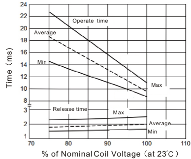
Operate Time/Release Time
