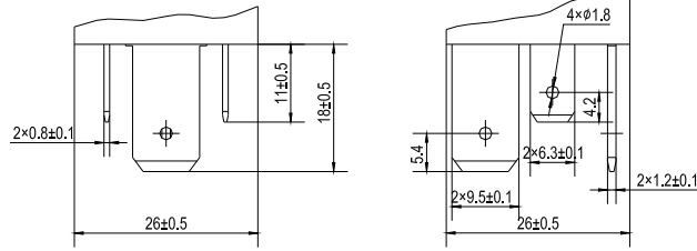
Plug in type Mounting (Bottom view)
