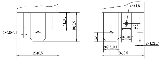
Plug in type Mounting (Bottom view)
