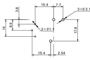
Double coils
