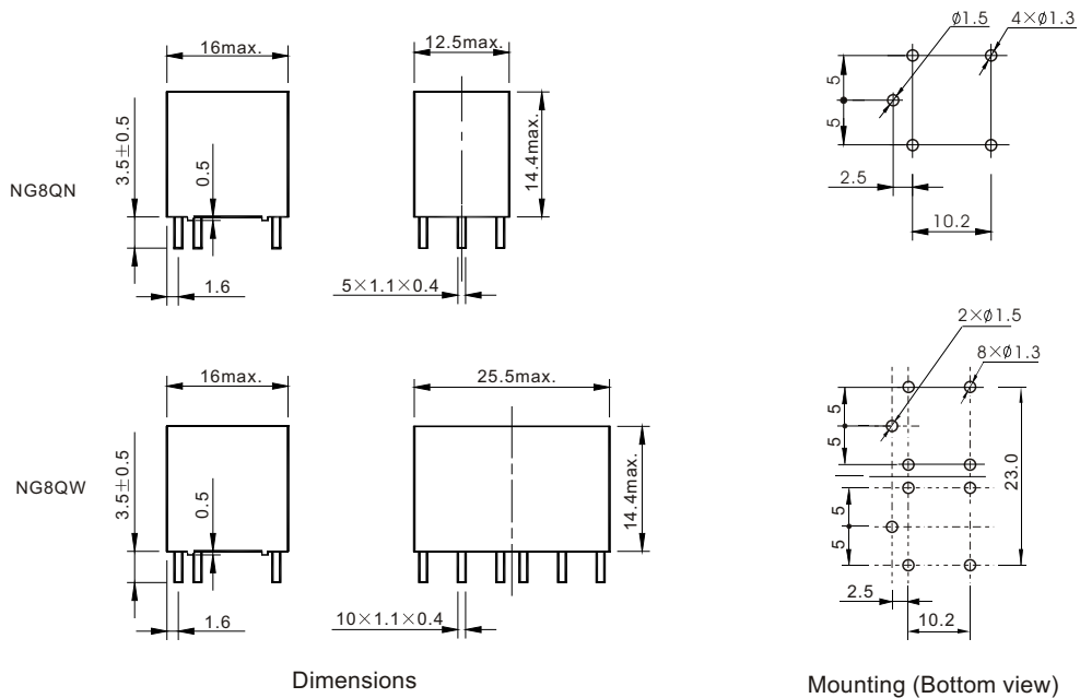
Mounting (Bottom view)
