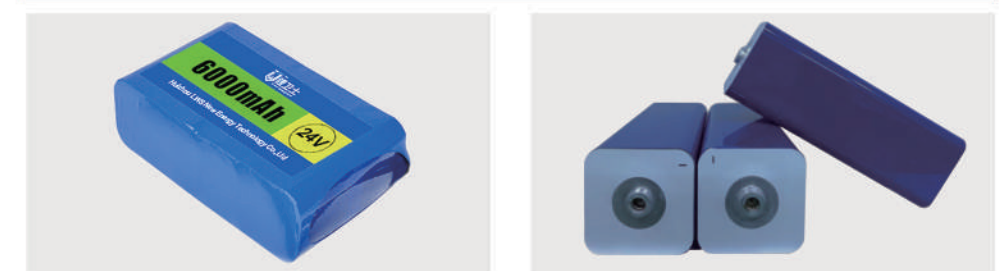
Rechargeable Lithium Battery Pack Voltage capacity:24V6Ah Size: 114*41*72mm Weight: 586g
