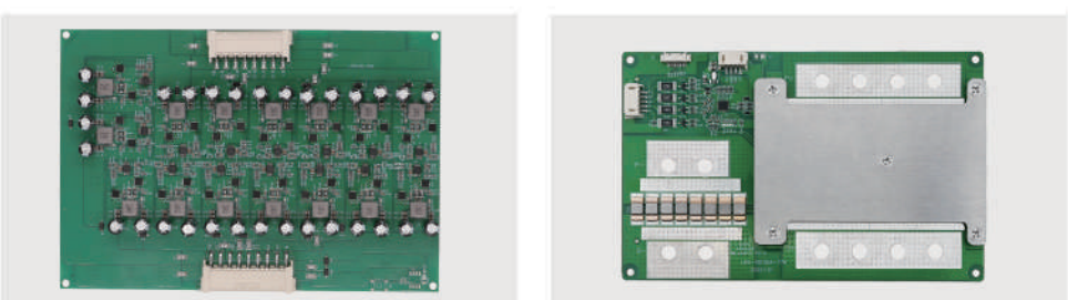
Model: LWS-BL-16S Size: L160*W110*T15mm Balance current: 2A Model: LWS-4S150A-779 Size: L155*W100*T16mm Charge/Discharge: 150A
