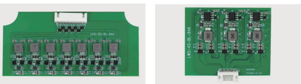
Model: LWS-8S-BL-844 Size: L105*W50.5*T8.5mm Balance current: 1A Model:LWS-4S-BL-846 Size:L50.1*W40.1*T10mm Balance current: 2A
