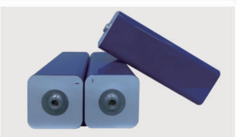
Rechargeable Lithium Battery Pack Voltage capacity:24V6Ah Size: 114*41*72mm Weight: 586g
