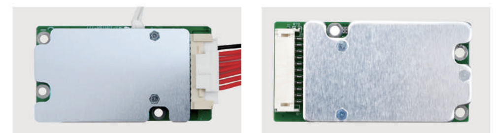
Model: LWS-10S15A-777 Size: L62.5*W34*T9.5mm Charge/Discharge: 15A Model: LWS-10S15A-611V1 Size: L60*W32.5*T9.5mm Charge/Discharge: 15A
