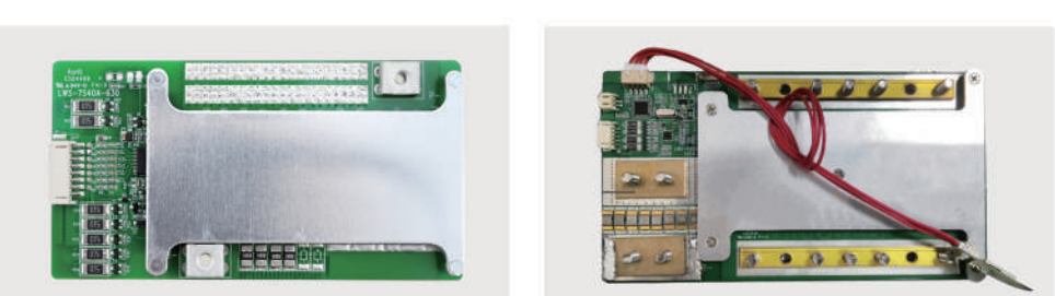
Model: LWS-7S40A-630 Size: L152*W76.5*T12mm Charge/Discharge: 40A Model: LWS-4S200A-774 Size: L193*W110*T15mm Charge/Discharge: 200A
