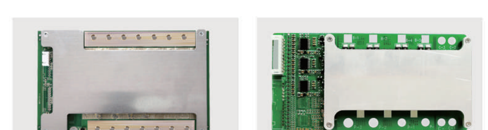
Model: LWS-20S300A-482 Size: L175*W116.5*T18mm Charge/Discharge: 300A Model: LWS-24S100A-444 Size: L125*W63*T10mm Charge/Discharge: 100A
