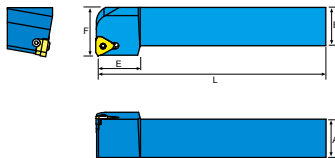
螺紋車刀架 Threading Tool Holder
