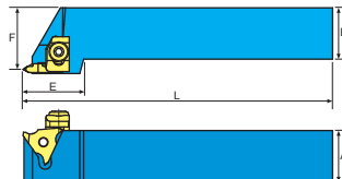
Threading Tool Holder
