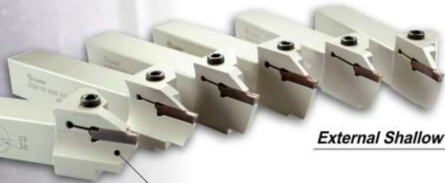
External Grooving
