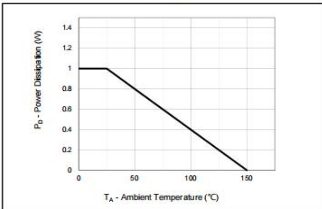
Fig.5 - Power Dissipation Derating Curve
