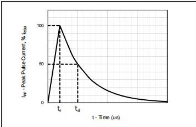
Fig.3 - Pulse Waveform
