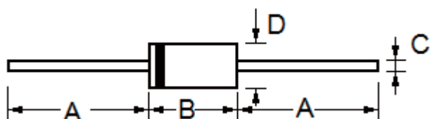
DO-201AE
