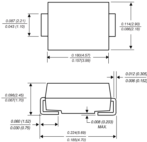
DO-214AC
