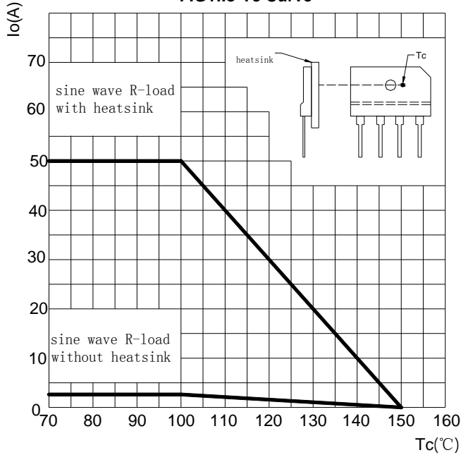
FIG1:Io-Tc Curve
