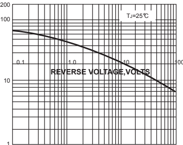
FIG. 5-TYPICAL JUNCTION CAPACITANCE
