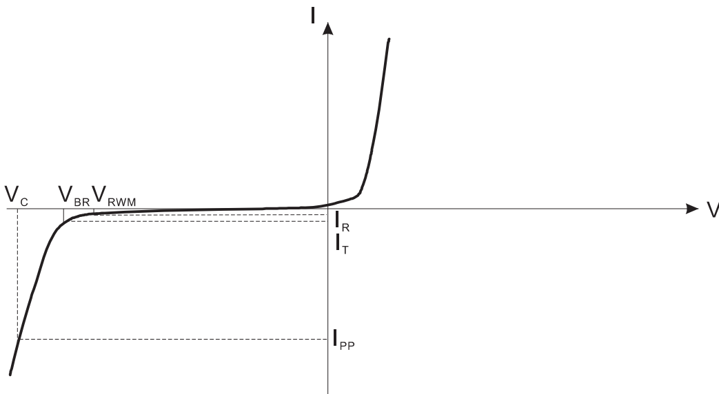
Uni-Directional TVS
