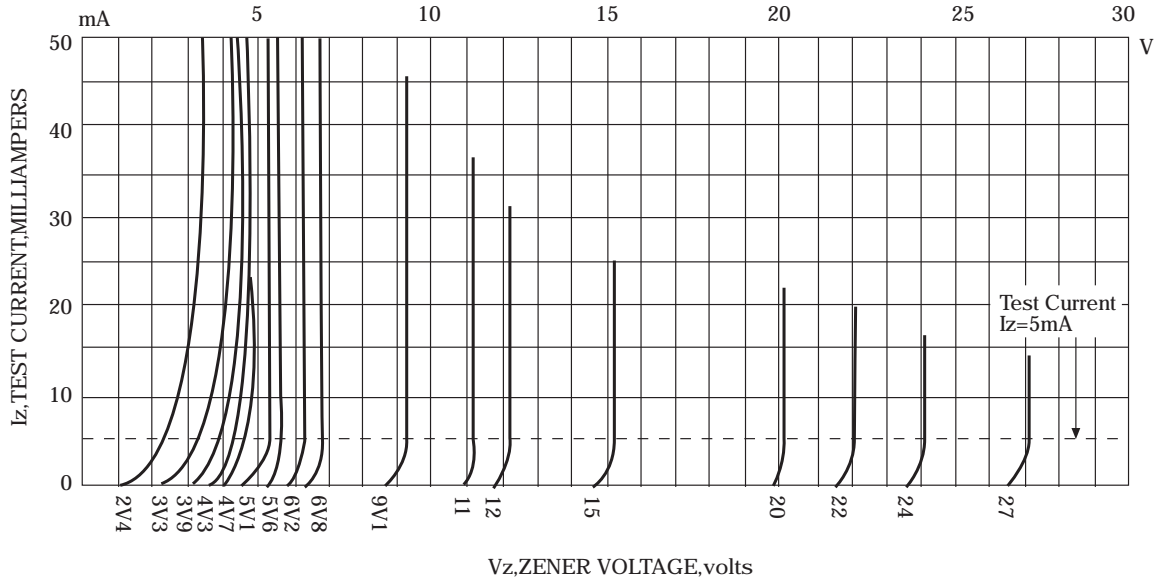
Breakdown characteristics
