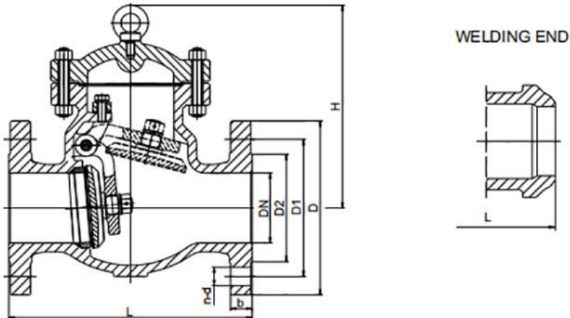
DIMENSIONS(mm) Class150
