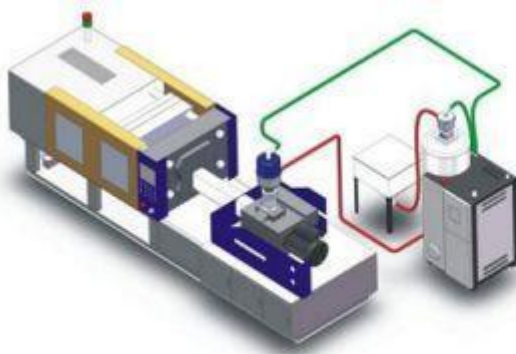
1对1 二段送料示意图 (标准) For Serving One Machine Two-stage Conveying System (Standard)
