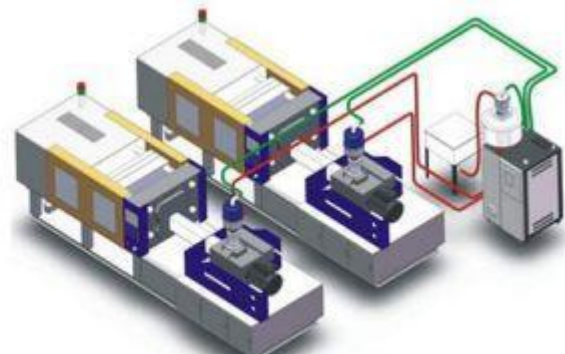
1对2 三段送料示意图 (选配) For Serving Two Machines Three-stage Conveying System (Optional)
