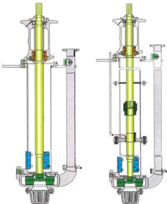
CANTILEVERED SHAFT
