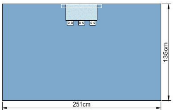
PM6103 Top Drape - 23x50cm Absorbent Reinforcement - Instrument Pad - Tube Holders
