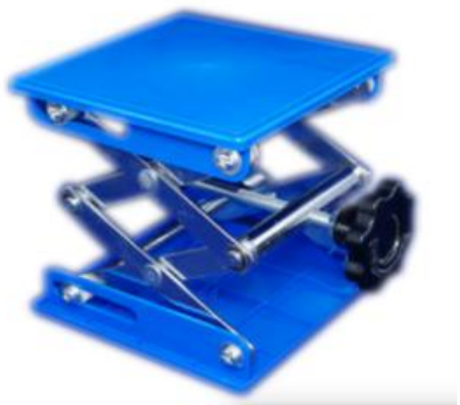
HSG-203 Lab jack 15*15*25CM Stainless body ABS board
